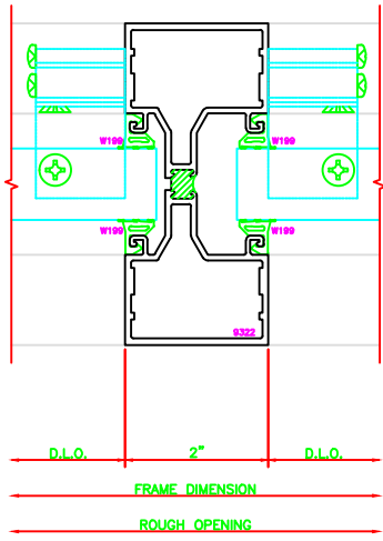
608 STANDARD VERT. 403 SHEARBLOCK
