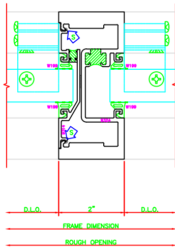
611 HEAVY DUTY VERT. 403 SHEARBLOCK
