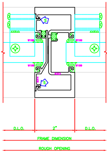
610 HEAVY DUTY VERT. 403 SHEARBLOCK
