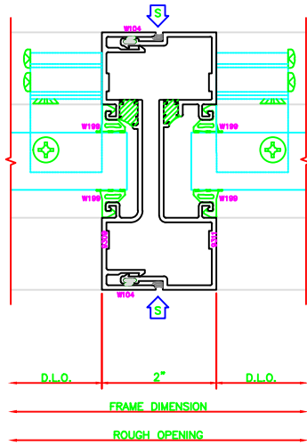
628 EXPANSION VERT. 403 SHEARBLOCK
